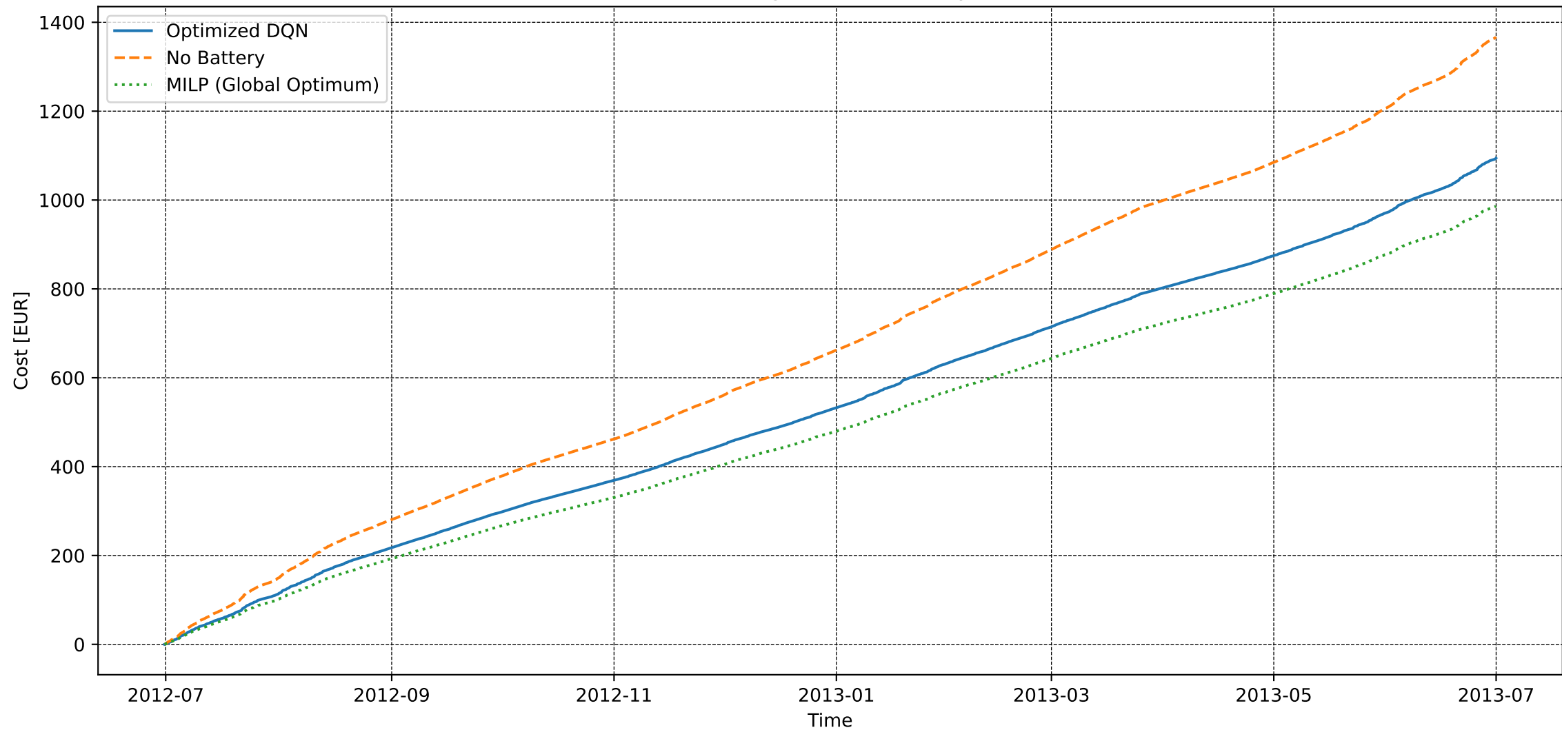
User 65 - Extended Convergence - Electricity Cost [DQN vs MILP]
